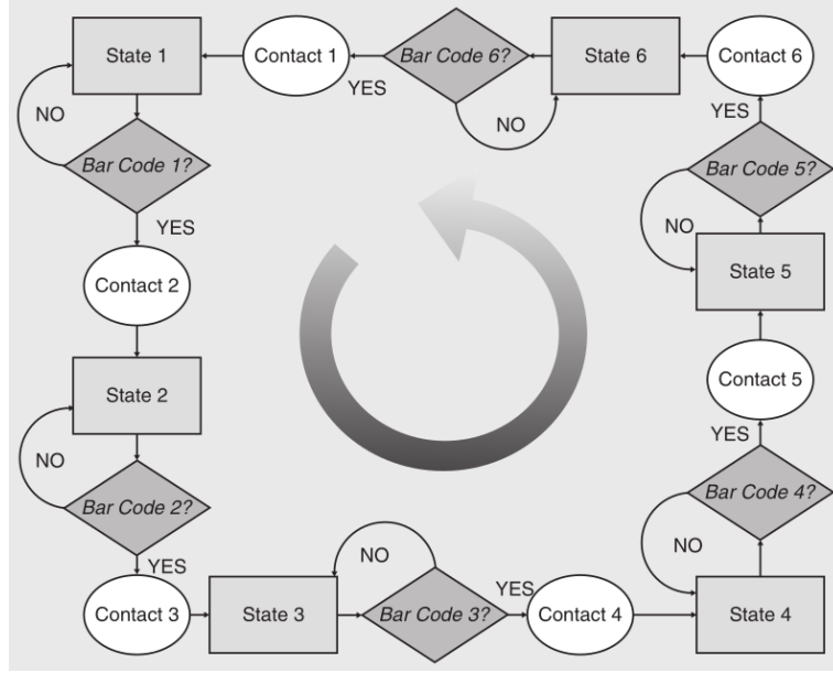
Figure 2.7: State diagram shows behaviors of the robot according to the sensor inputs
