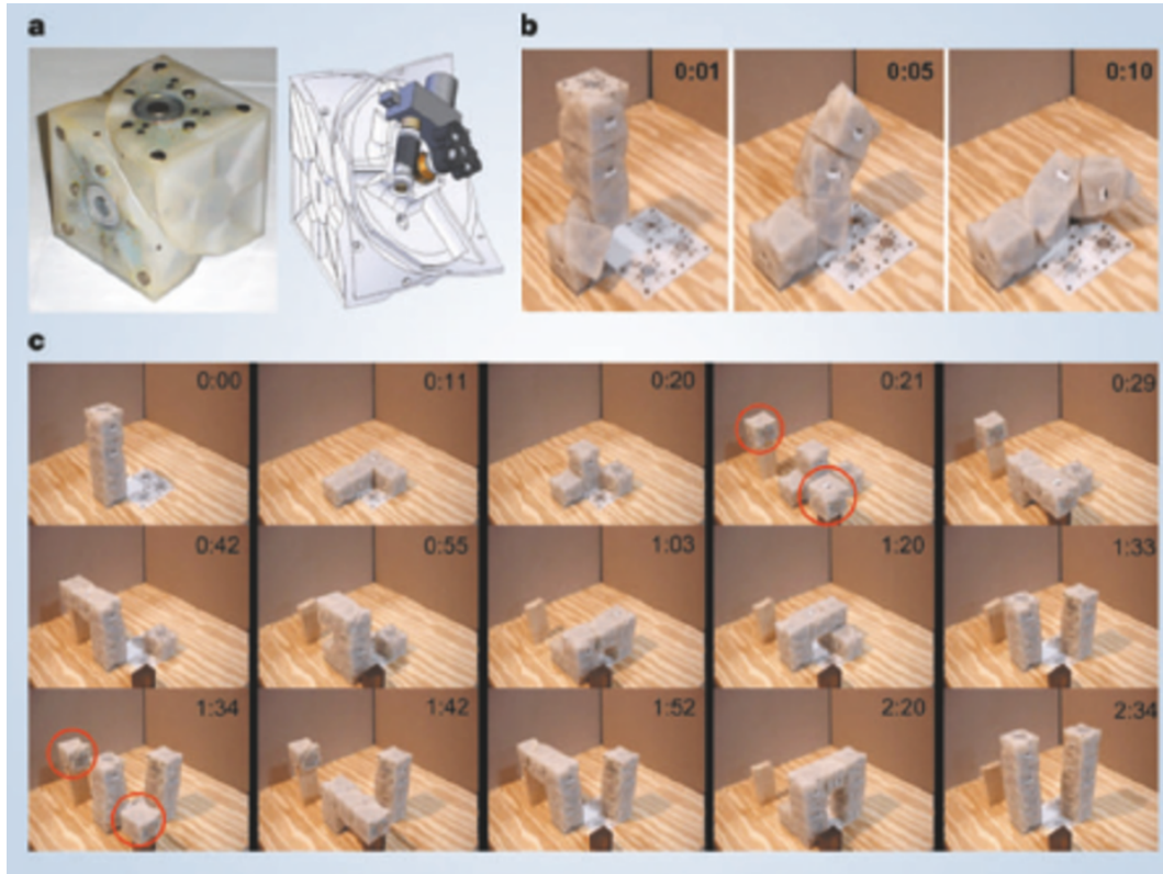
Figure 2.8: Self-replication of a four-module robot
